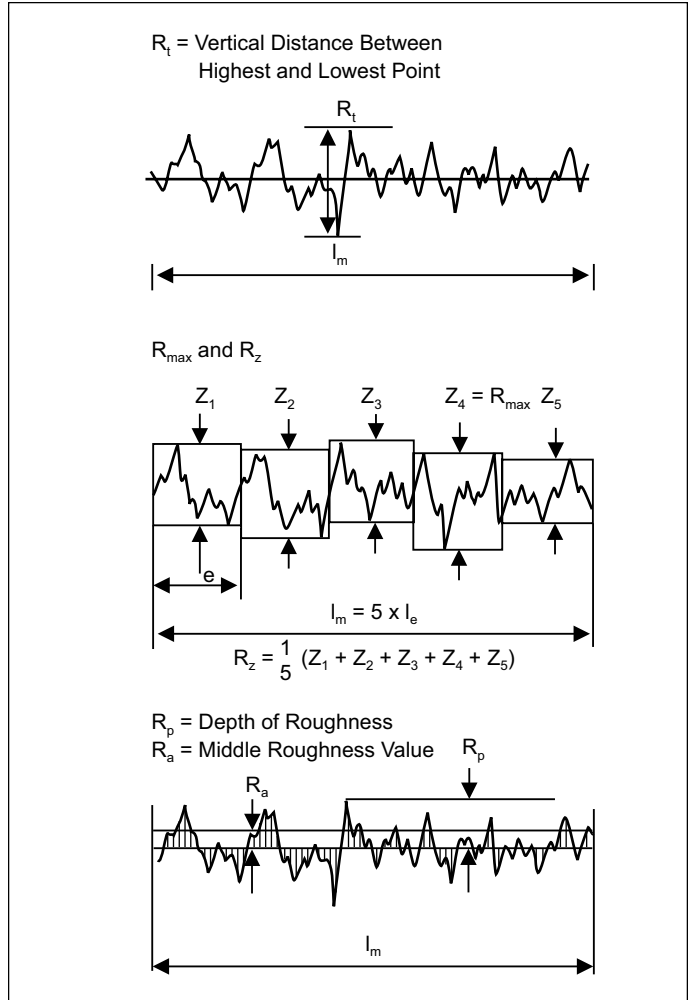
Figure 5-4: Roughness Terminology
