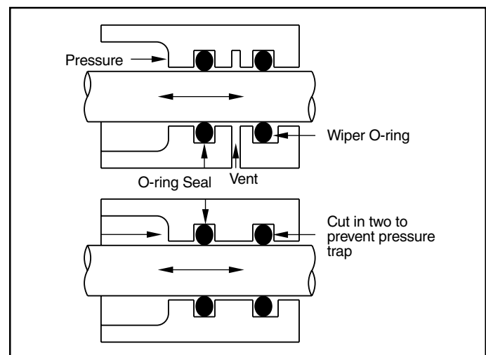
Figure 1-14: Wiper Installation
