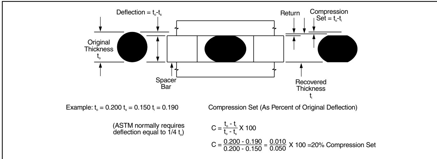
Figure 2-9: Compression Set
