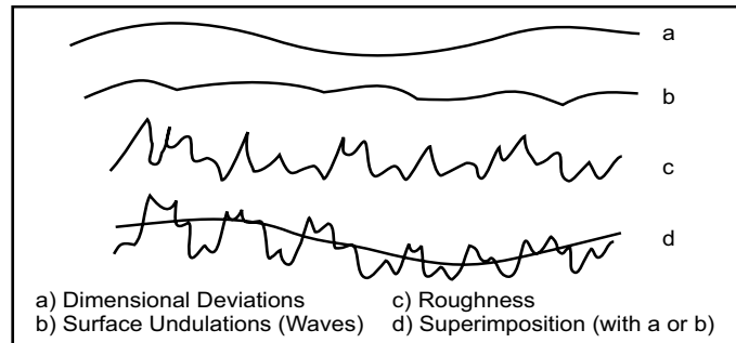
Figure 5-3: Surface Finish Structure
