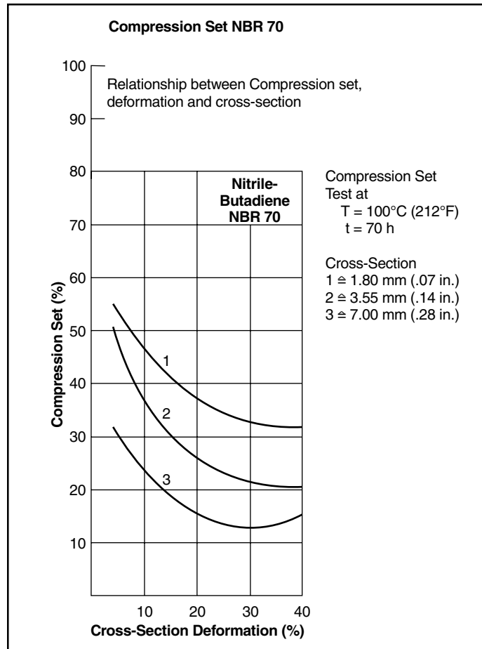
Figure 2-11: Compression Set NBR 70
