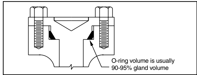
Figure 1-13: Crush Installation
