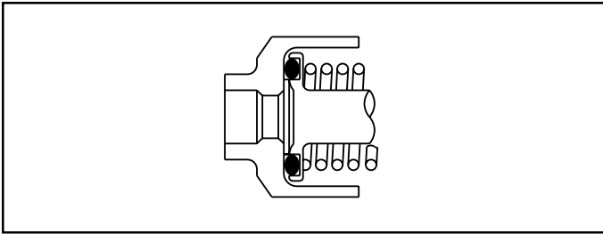
Figure 1-12: Seat Seal
